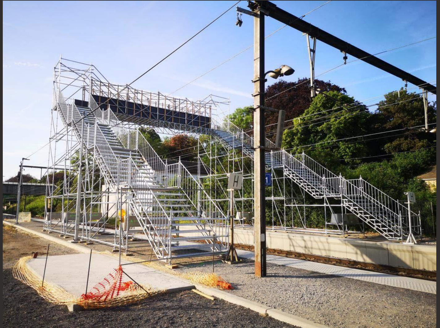
Walkway, MetalScaff, BE
