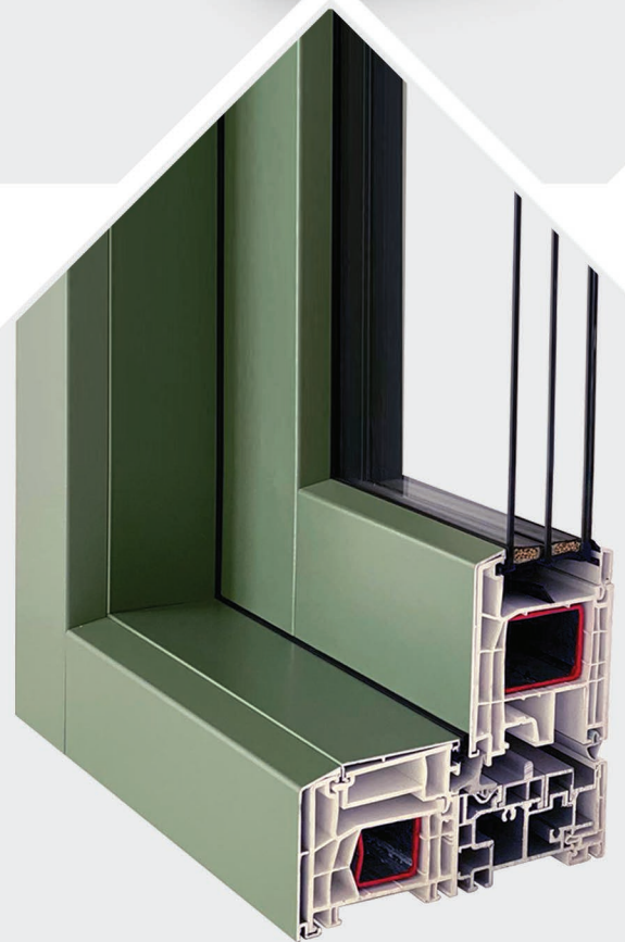
Premislide - uPVC sliding door profile 1 of 4 available profiles
